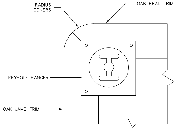
DETAIL AT BACK OF BOARD SHOWING TYPICAL CORNER WITH KEYHOLE HANGER. SCALE= 1/2 FULL SIZE
