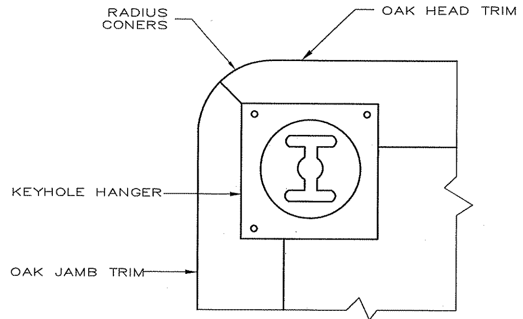
DETAIL AT BACK OF BOARD SHOWING TYPICAL CORNER WITH KEYHOLE HANGER. SCALE= 1/2 FULL SIZE
