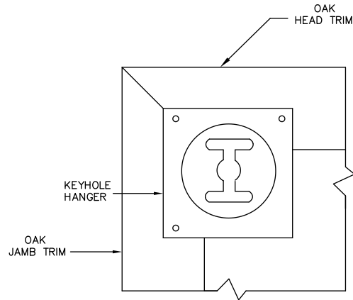
DETAIL AT BACK OF BOARD SHOWING TYPICAL CORNER WITH KEYHOLE HANGER. SCALE = 1/2 FULL SIZE
